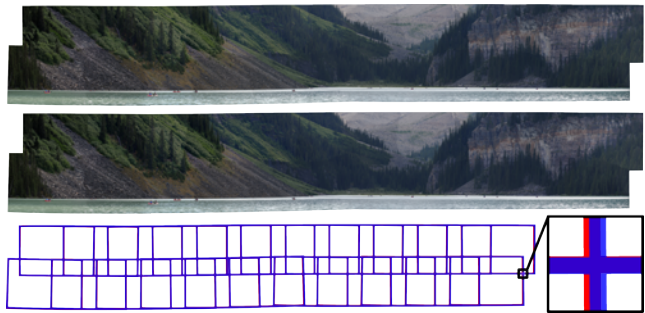
Fig. 4. Comparison between a registration obtained with our preview (top) and a full (middle) bundled adjustment. The registration of the last image took 0.181 and 15.046 seconds for the preview and full computations respectively (149 megapixel, 22 images). Bottom: layout of the boundary of the images for the two solutions (transparent blue: preview, red: full).
